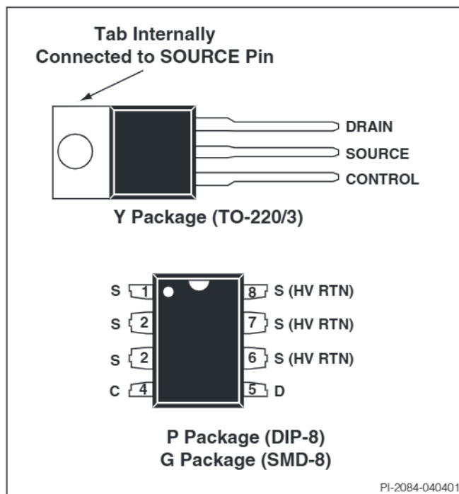
Figure 3. Pin Configuration.
