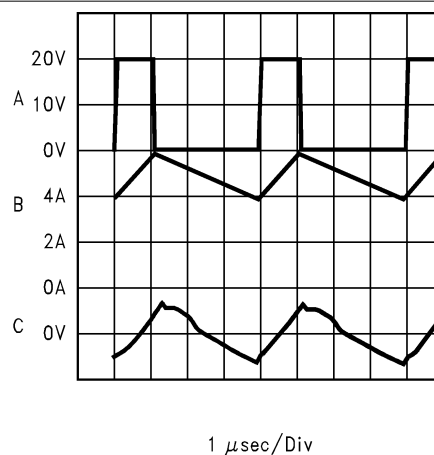
Figure 5-10. Switching Frequency
