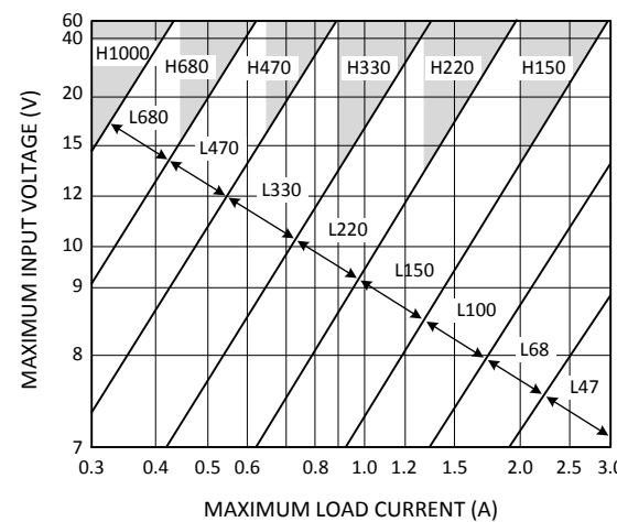
Figure 22. LM2576-5.0
